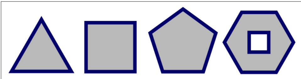
Figure 15-8. Regular polygons
